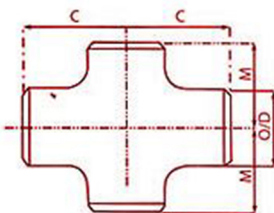
CROSS UNEQUAL
